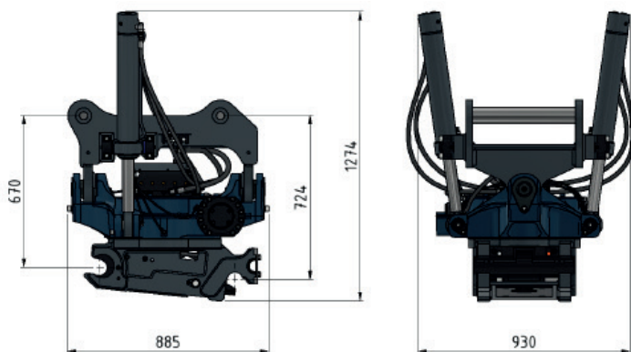
Dimensions for ST32 with S70 Hardlock
