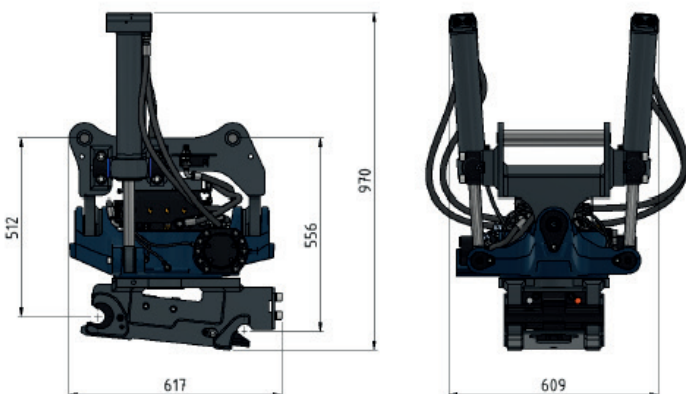
Dimensions for ST10 with S45 Hardlock
