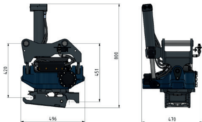
Dimensions for ST6 with S40 Safelock
